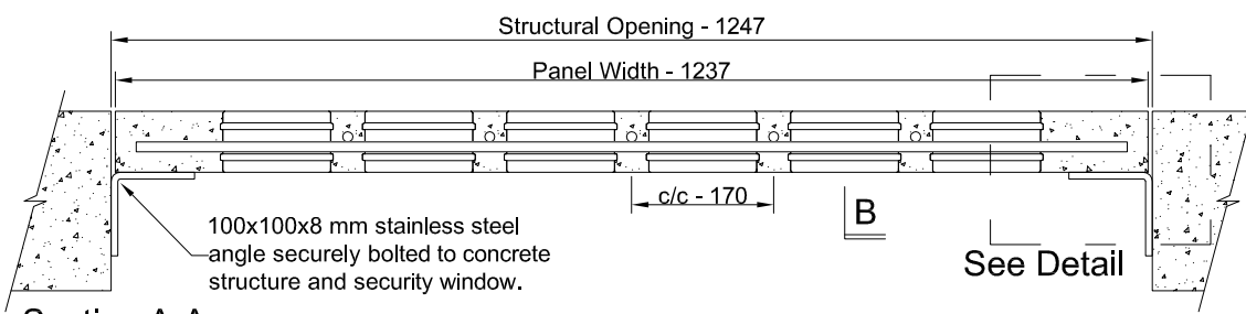
Section A-A Scale 1:10
