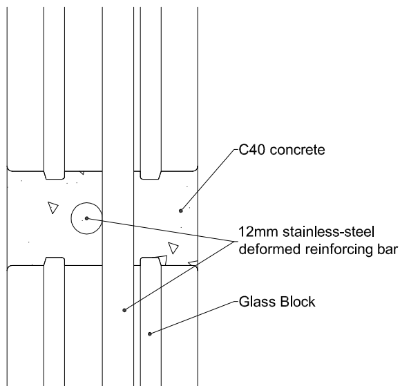
Typical Mortar Joint Scale 1:2
