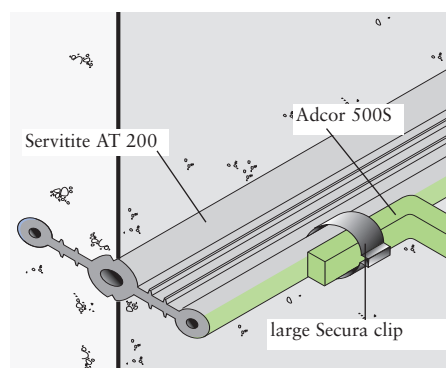
Adcor® 500S attached to Servitite® AT 200 at Movement Joint
